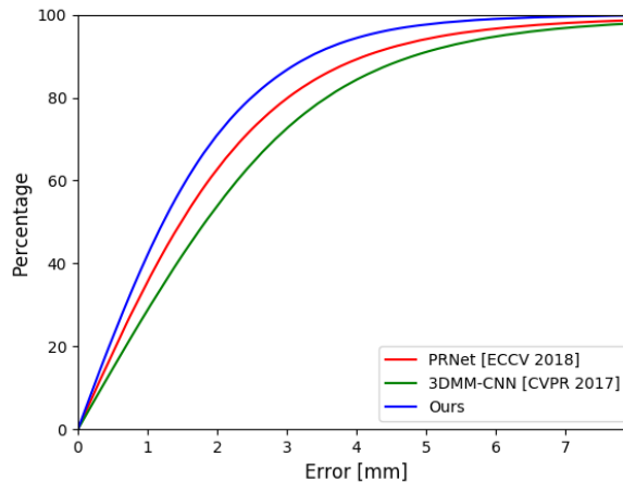
Figure 9: Cumulative error curves for expression challenge.
