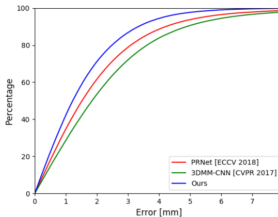
Figure 10: Cumulative error curves for occlusion challenge.
