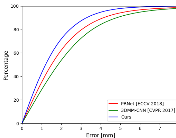
Figure 11: Cumulative error curves for selfie challenge.
